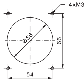
Bohrplan M10, M20
